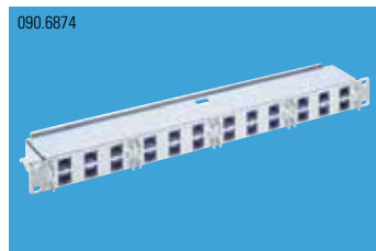
19" 1U HD Basic Patch Panel 24xRJ45/s, Real10 Cat.6, gray, fully populated
