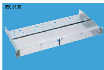
19" 1U HD Patch Panel 48-Port, gray, empty
