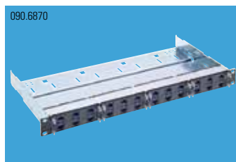
19" 1U HD Patch Panel 24xRJ45/s, Real10 Cat.6, black, fully populated
